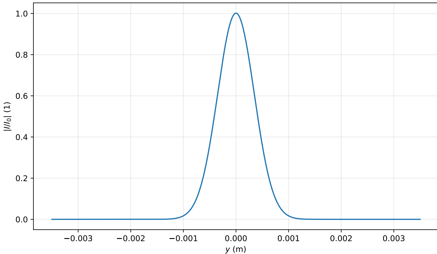
Intensity profile I(x=0, y, z=0.080)/I_0 , \text{Pin}=0.5\text{Pcr} , artificial time
